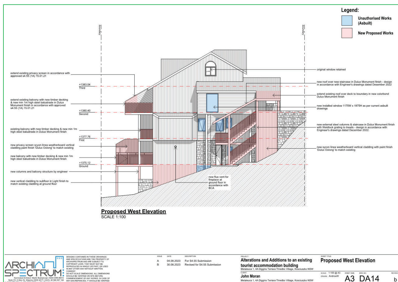
Figure 3-9 West elevation.
