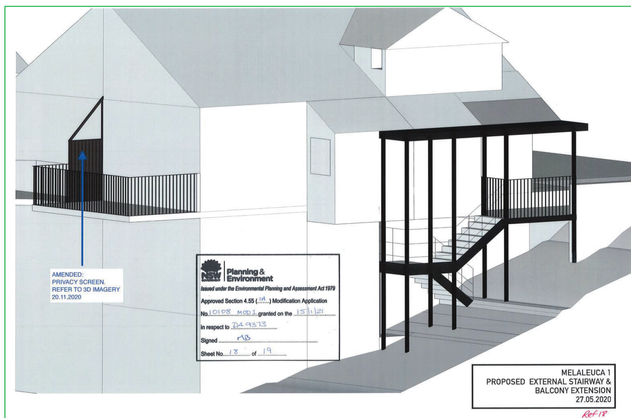
Figure 3-3 External view - privacy screen, proposed external stairway and balcony extension.
